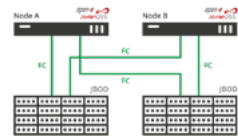
Cluster with multiple JBODs over SAS/FC (with ATTO bridges)
